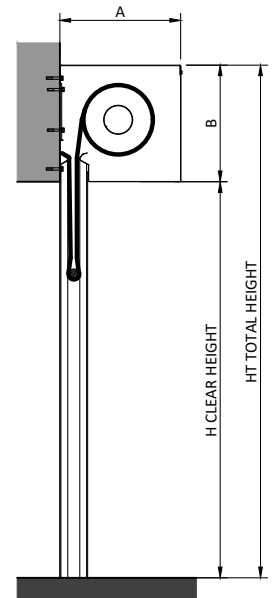
TYPICAL SECTION FACE FIXED
