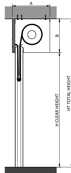
TYPICAL SECTION FIXED BETWEEN
